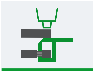
ADO connection (IDC connection technology)
